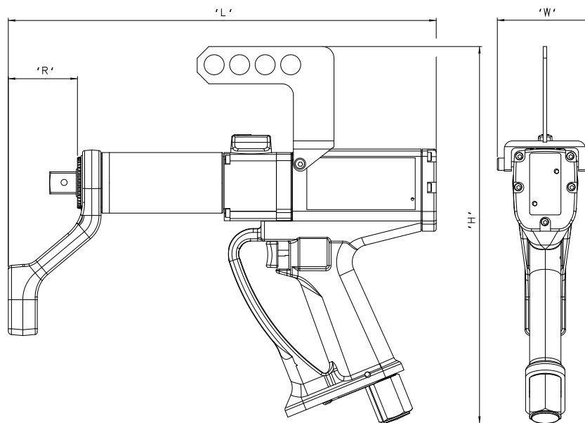
FIGURE 9 – Tool Dimensions
